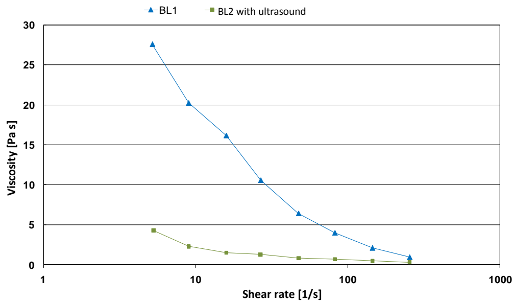
Figure 3: Viscosity of the biomass in the digester
